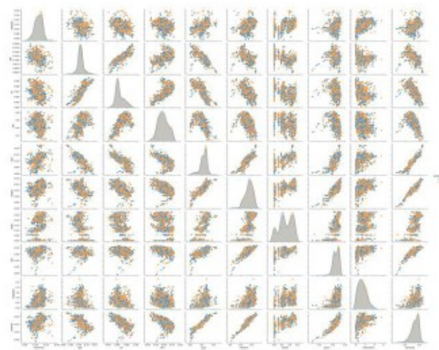
fig1: Pair plot of selected acoustic features separated by gender.
