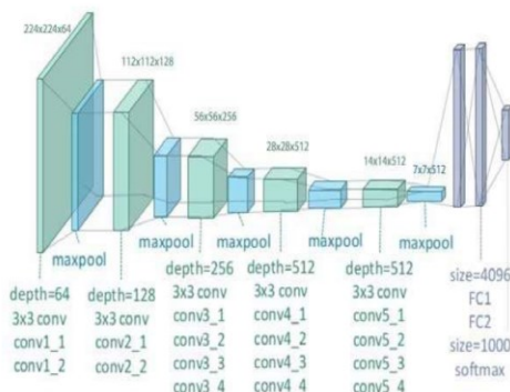
VGG-19 architecture
