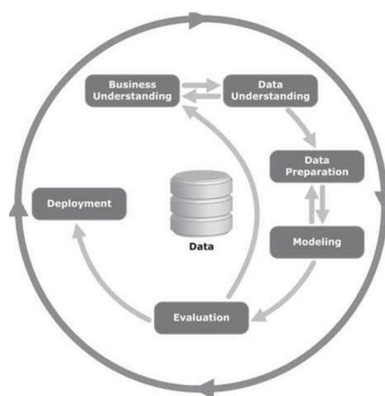
Fig. 3. Process diagram
