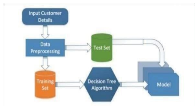
Fig. 5. Architecture Diagram
