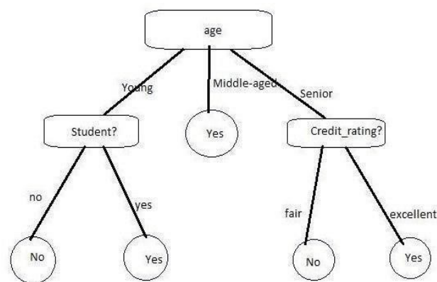
Fig. 2. Decision Tree
