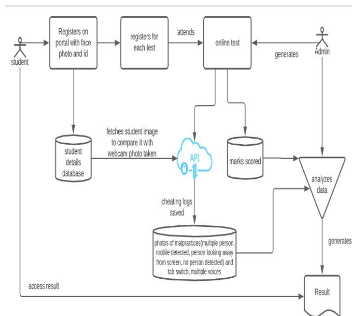
Fig 1. System Methodology
