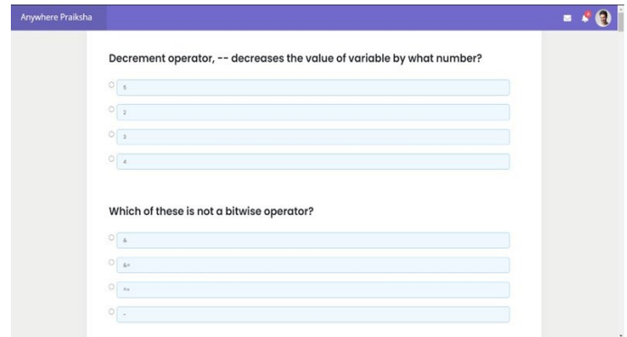
Fig 6. Test screen
