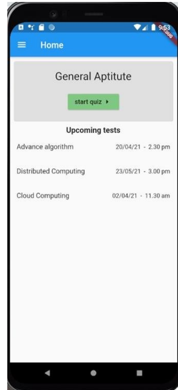
Fig 12 Mobile app
