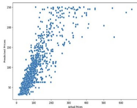
Fig-3 Random Forest performance.
