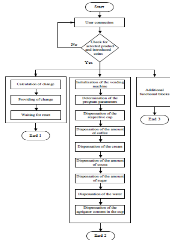
Fig. 2. A control algorithm.
