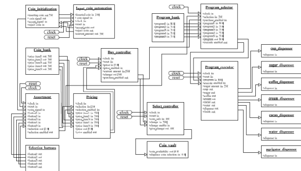
Fig. 1. A block diagram of the implemented vending system.
