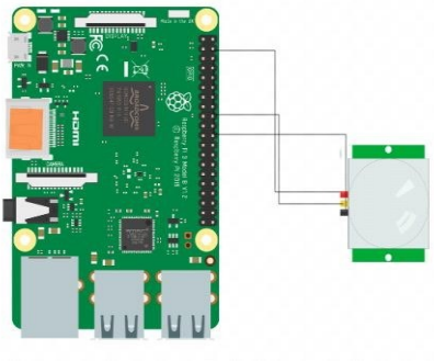
Fig:6 Raspberry pi with PIR sensor.
