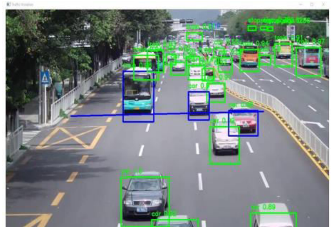
Fig.5. Vehicle classification.
