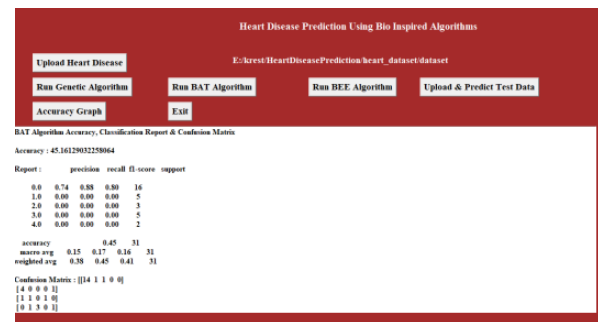
Fig.4. BAT Accuracy.
