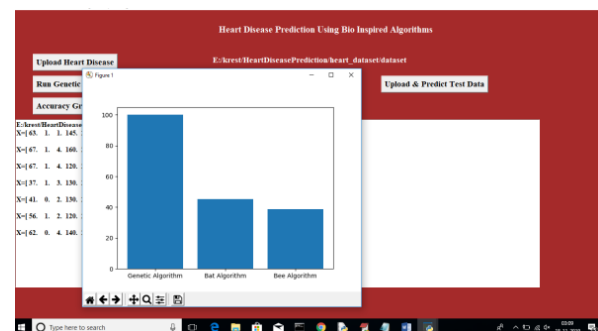
Fig.5. Accuracy Graph.
