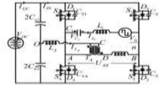
Fig. 4. Simplified network with battery load referred at transmitter coil side.
