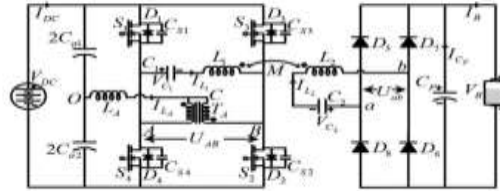
Fig. 5. Proposed network configuration of EV battery charger.
