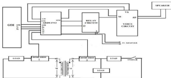
Figure 5 – Circuit Diagram Of This Proposed System
