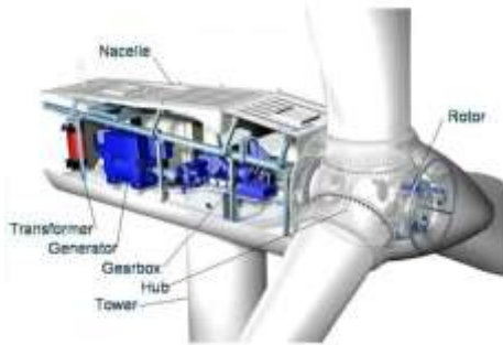
Fig.3 Cross section showing the arrangement of internal parts of a wind turbine
