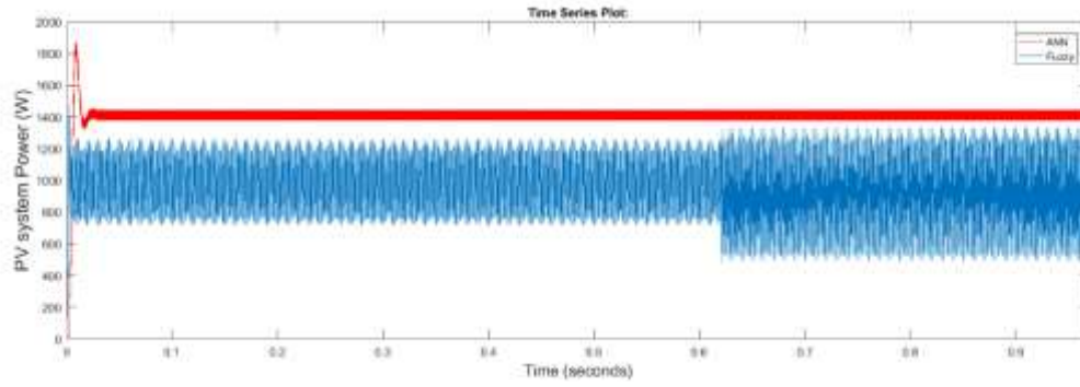
Fig6. PV system power(W) with the Fuzzy and ANN controllers
