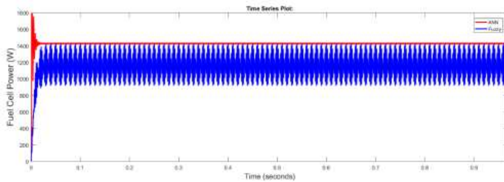
Fig8. Fuel cell power(W) with the Fuzzy and ANN controllers
