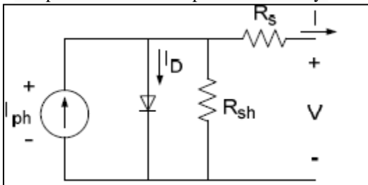
Fig 2. Equivalent circuit of solar array.
