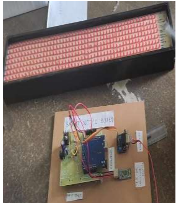
Fig: contact less notice board using Bluetooth
