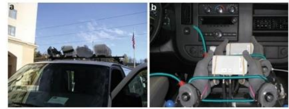
Fig. 8.1 (a) and (b) show the field trial in car roof and in the car, with and without hand phantoms (Courtesy of Ericsson AB)
