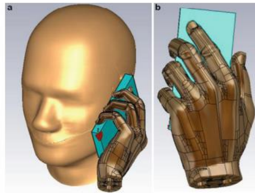
Fig.7 CTIA user cases: (a) talking mode and (b) data mode
