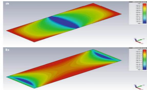
Fig. 6.1 Characteristic mode of mobile chassis: (a) E-fields, and (b) H-fields
