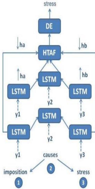
Fig. 2. The mechanism of the BLSTM-RNN method for classifying the relation of the sentence "imposition causes stress".
