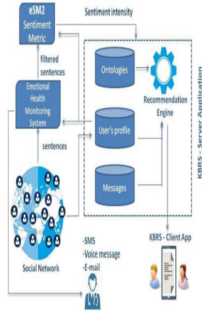
FIGURE 1: Architectonics of the proposed KBRS, which takes social network phrases into account.
