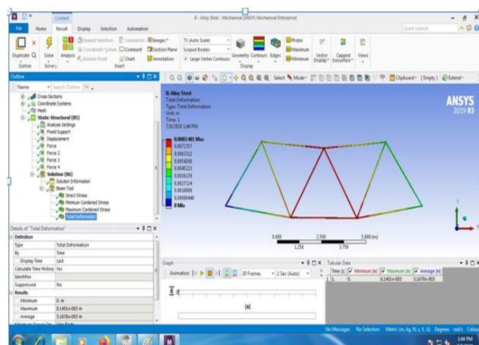
Fig.7.9 Total Deformation for Alloy Steel
