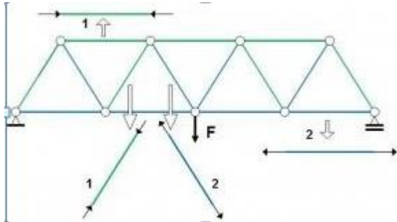
Fig1.1 Members under axial forces in a simple truss1 - Compression axial force
