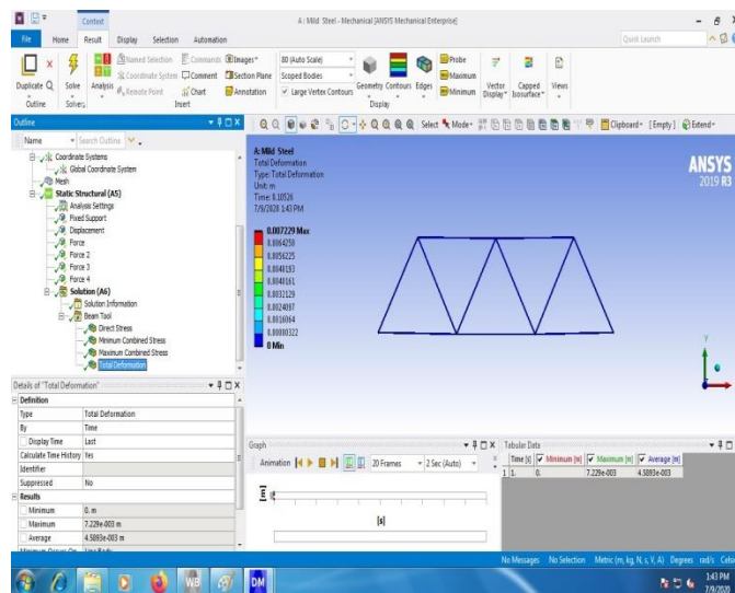
Fig.7.8 Total Deformation for Mild Steel
