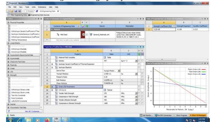
Fig 7.2 Engineering Data
