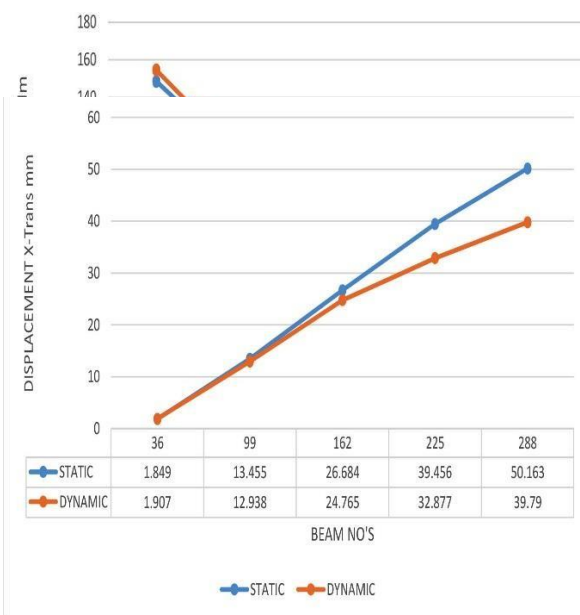
Graph 7. Static & dynamic analysis of Bending Moment in SMRF
