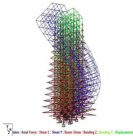
Fig.4 axial force, shear force, torsion and displacement
