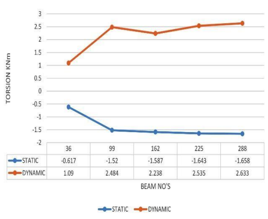
Graph 2.static & dynamic analysis of Torsion in OMRF
