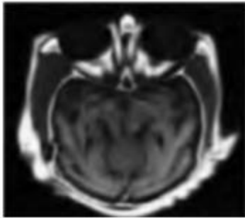
Figure 4.Pixel value maximization.
