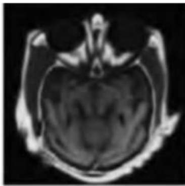
Figure 5.Wavelet transform method
