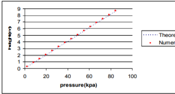
Figure4 Hydrostatic pressure variation along the height of water from theoretical and numerical methods
