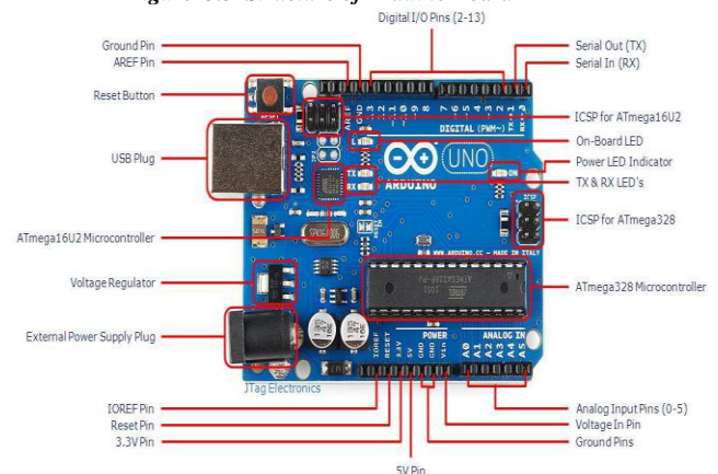
Figure3.4 Arduino Board
