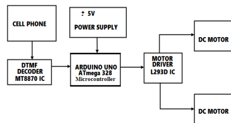
Block Diagram of Multi Terrain Robo
