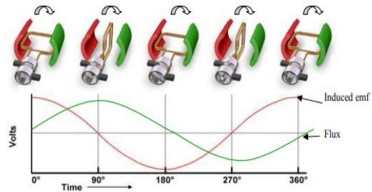
Fig 3.8 Production of alternating emfs in DC motor
