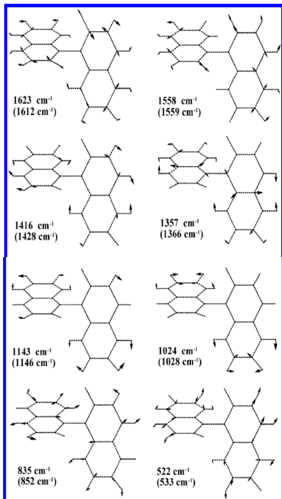
Figure 5. Schematic diagram showing the Cartesian displacements of selected Raman active modes of BN2- calculated with B3LYP/6-31G*.
