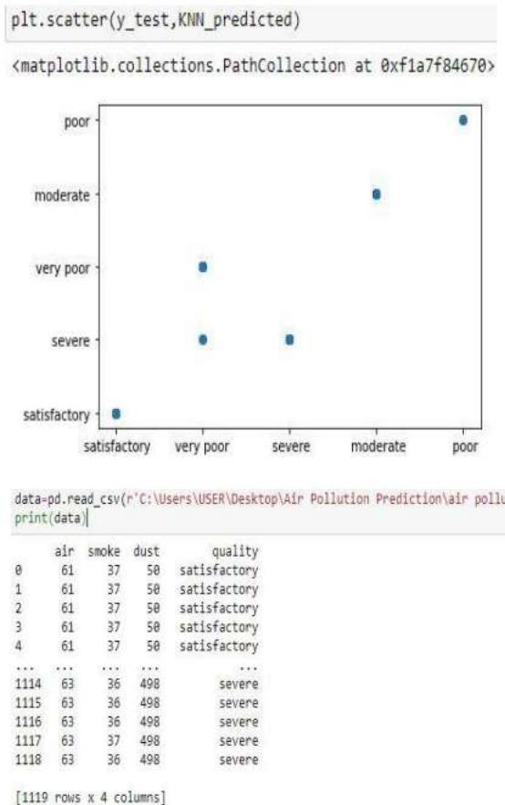
Fig.1. Dataset details.
