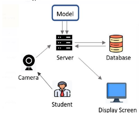
Fig.1. Architecture Diagram.
