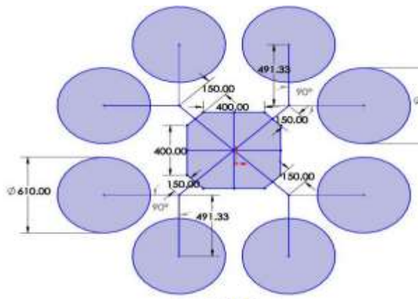
Fig -13: 2D Drawing
