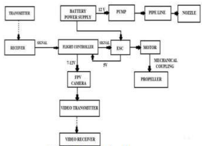
Fig -1: Block diagram of working process
